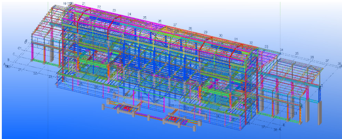
Mill building-model
